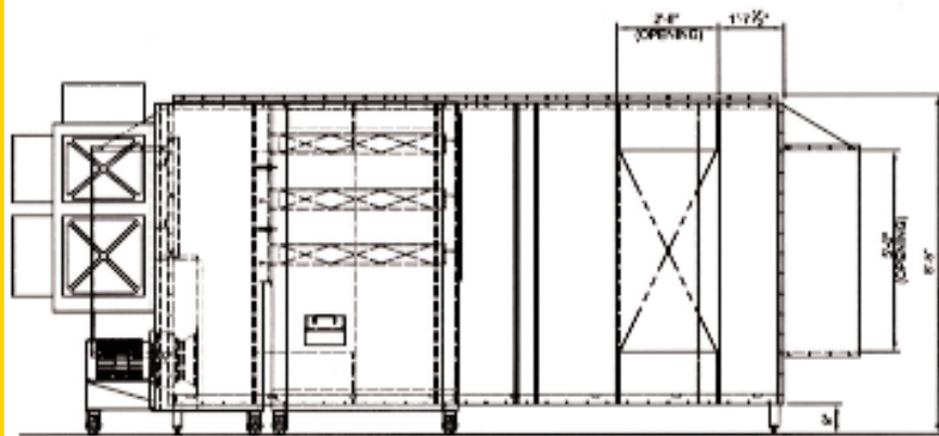
COLLECTOR SIDE VIEW
