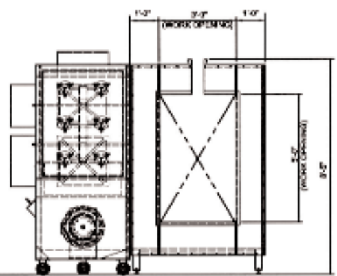
COLLECTOR ELEVATION
